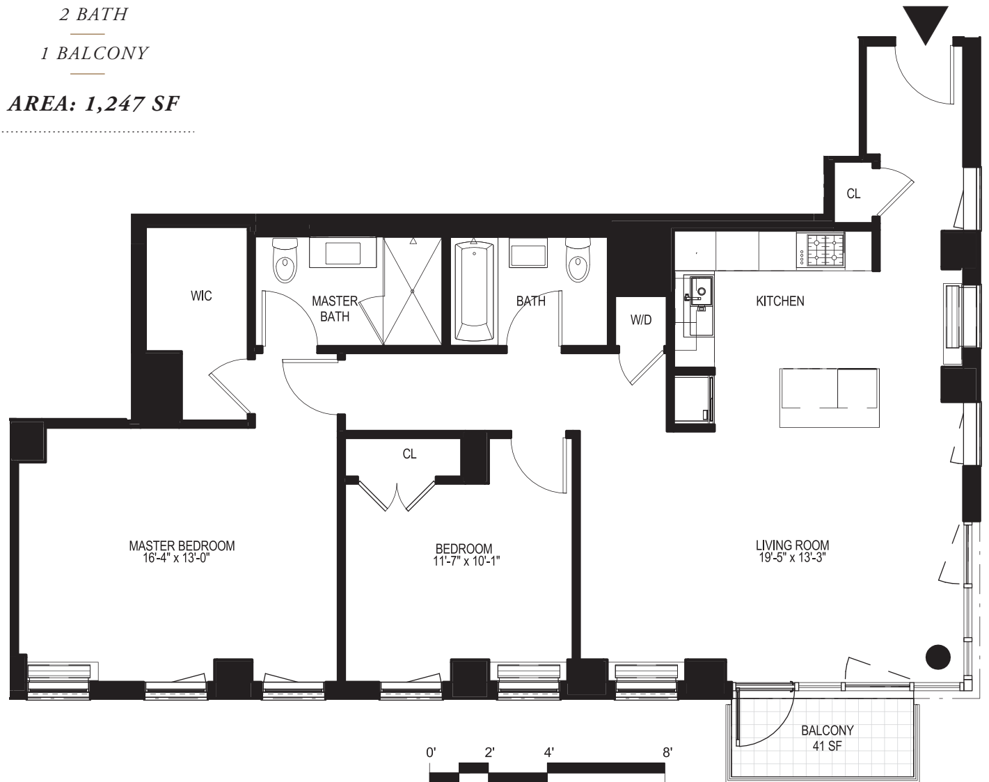
KEY PLAN
